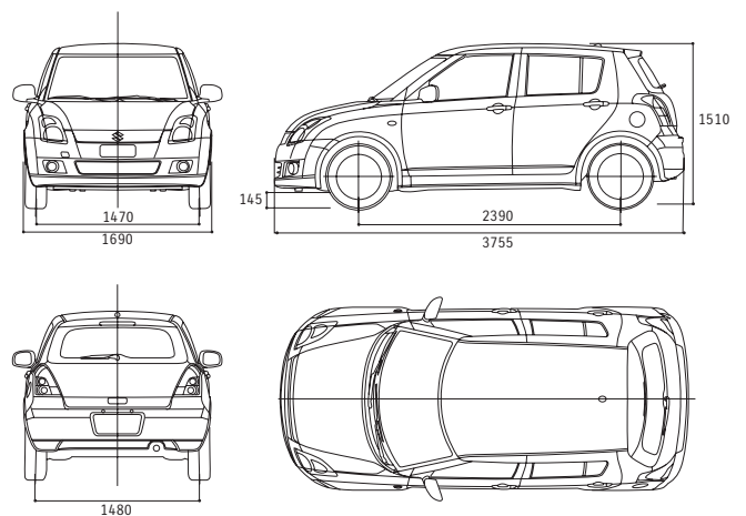
Dimensions (mm)
